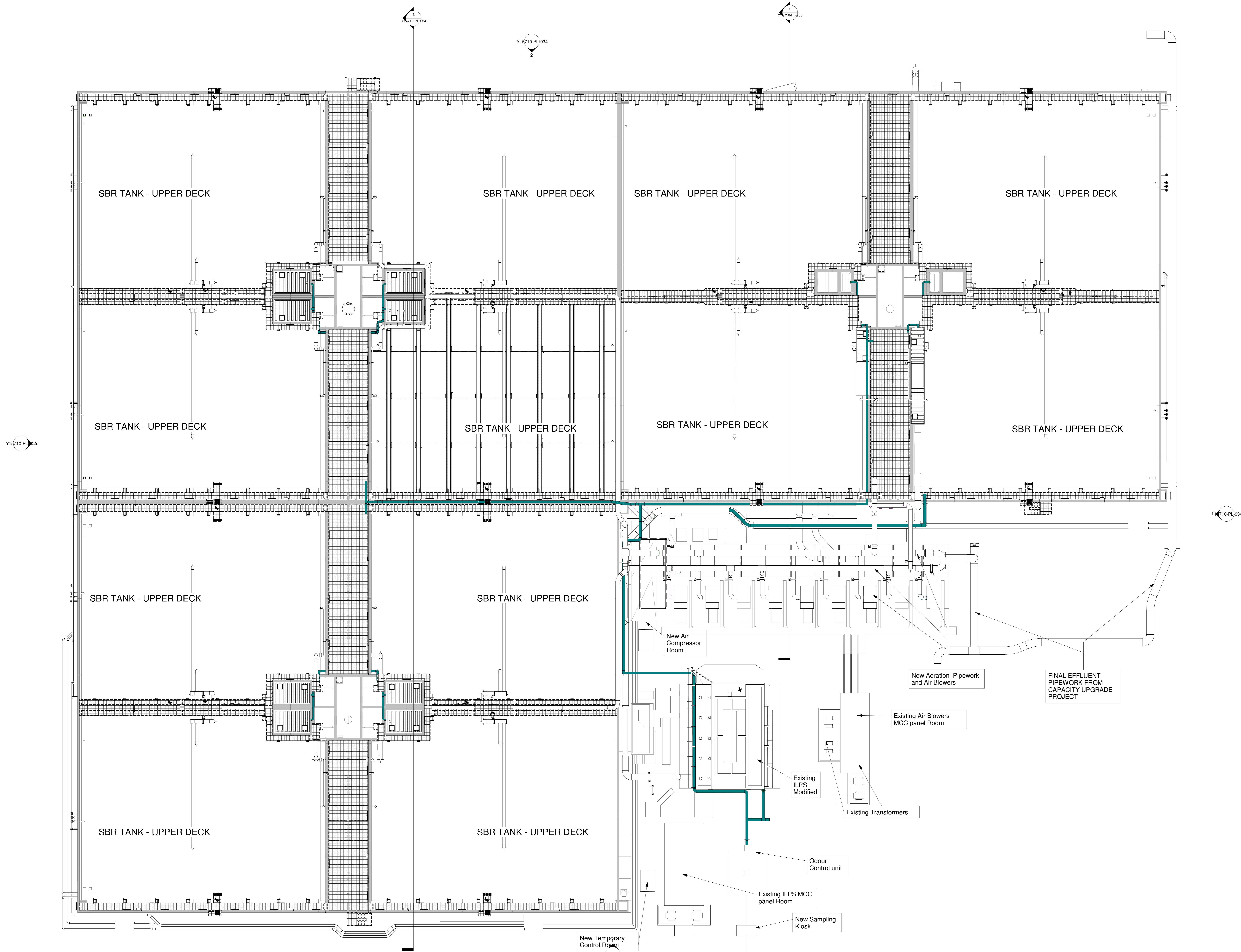
PROPOSED SBR RETROFIT @ 25.00m AMD 1 : 250
